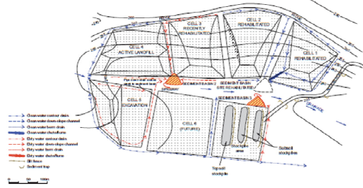
Figure B.3 Site layout and drainage plan - year 10
