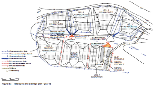
Figure 8.6 Site layout and drainage plan – year 15
