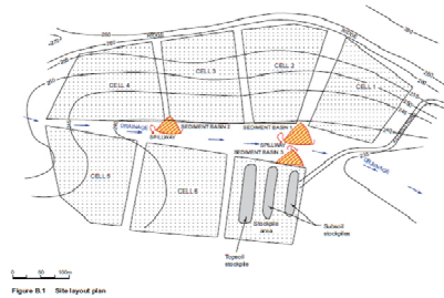
Figure B.1 Site layout plan
