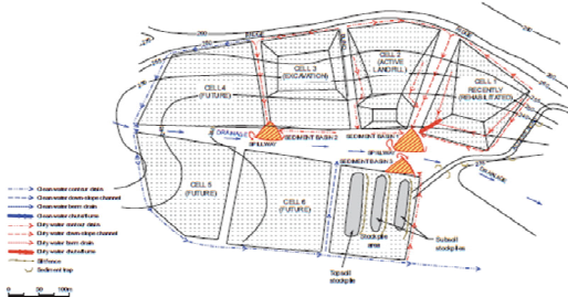
Figure B.2 Site layout and drainage plan - year 5
